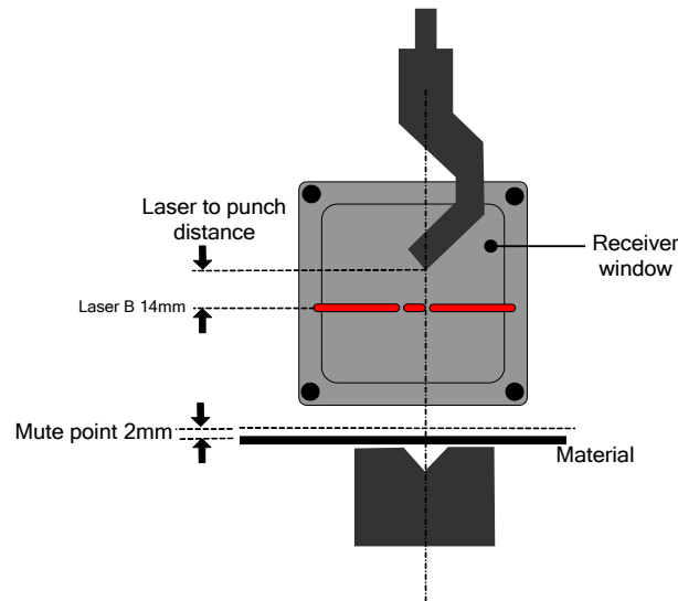
Figure 4-2: Laser to Punch Distance
