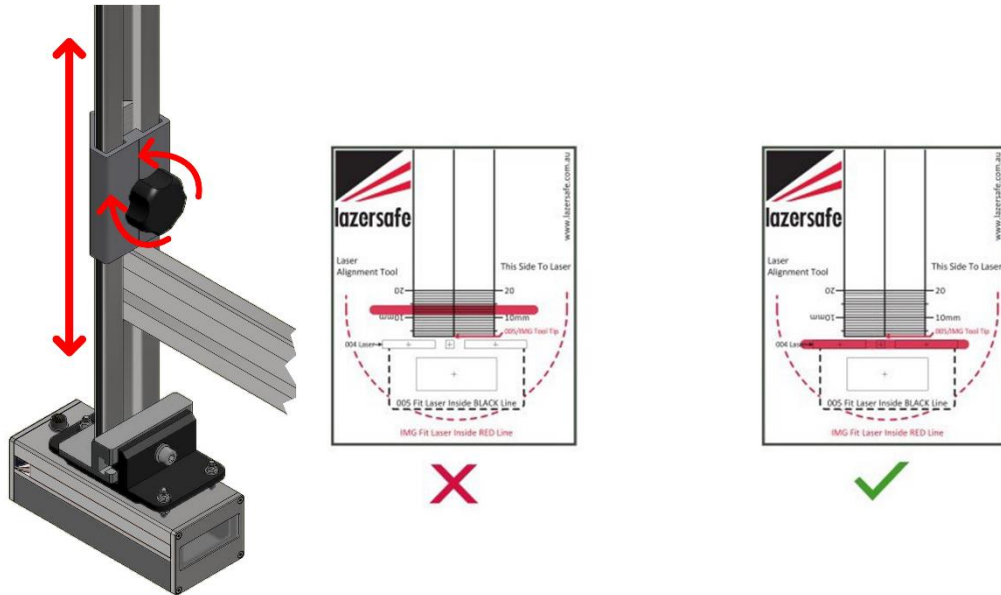
Figure 4-5: Vertical Bracket Adjustment
