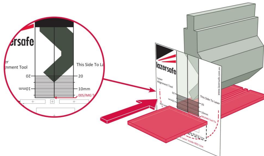
Figure 4-4: Fitting the Alignment Card to the Punch
