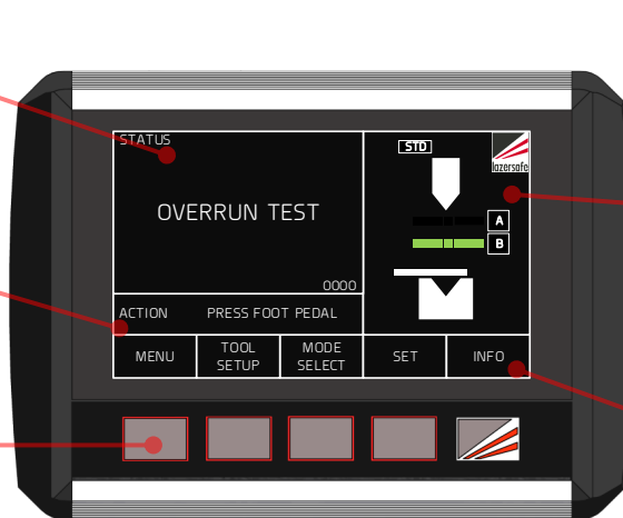
Figure 5-1: Defender Plus User Interface Panel
