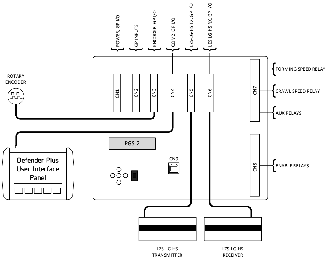
Figure 3-2: Defender Plus Press Brake Guarding System Components
