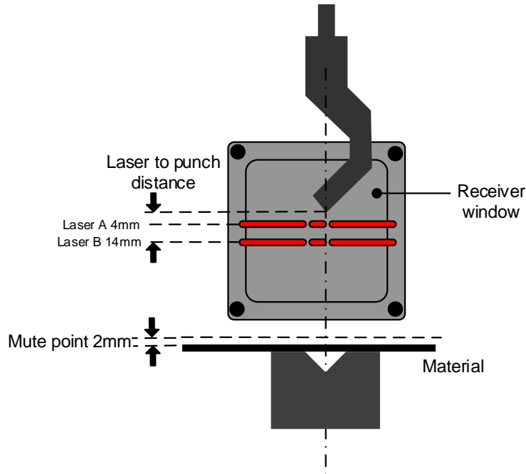
Figure 3-3: LZS-LG-HS Dual Laser
